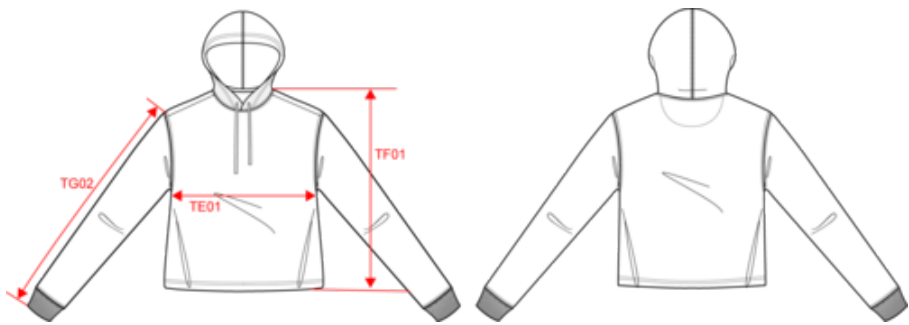
Dimensions (cm)
